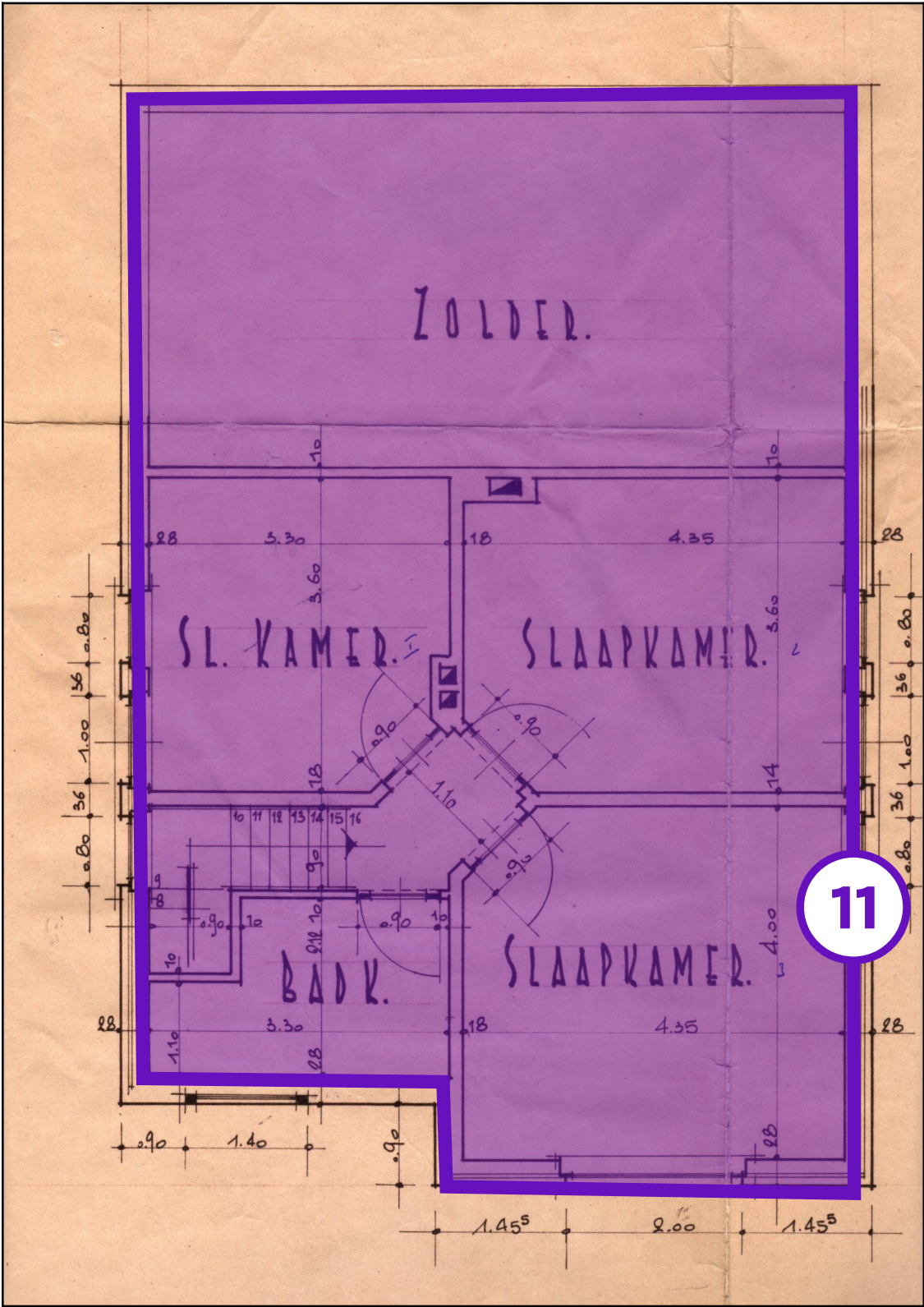
Legende van plan 1.6: verdieping 1d
